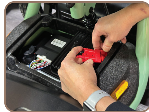
Plug the red anderson plugs together and replace the rear floor panel
