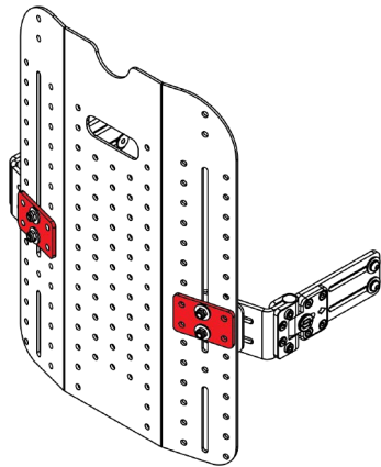
Reinforcement Plate 1266-2450-100
